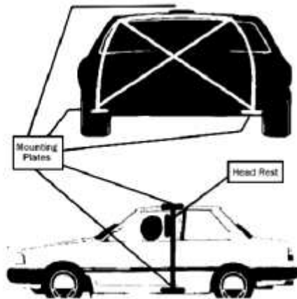
Pictured: Roll bar as required in Teams Derby Rules D2-1-5 to D2-1-10
